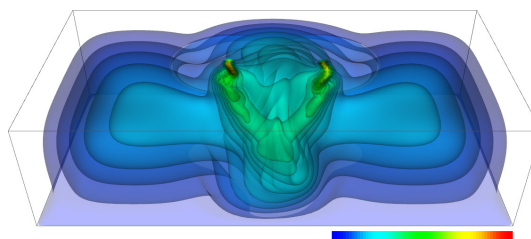
Figure 16: Temperature field at 10 ms
