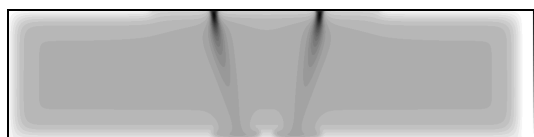
Figure 12: Projected temperature field at 1.0 ms
