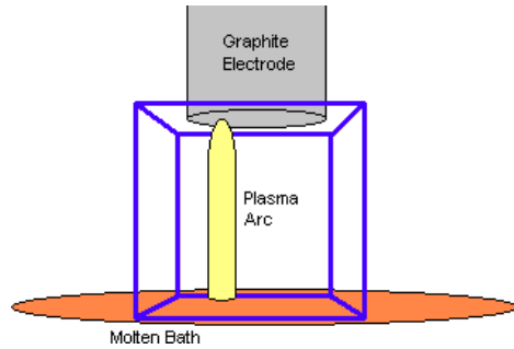
Figure 3: Solution region for arc models
